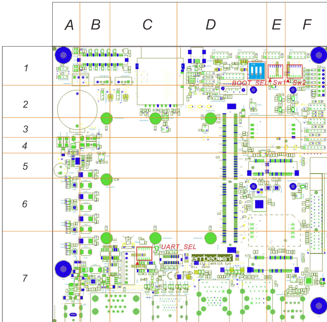
Figure 6: Switch Locations
