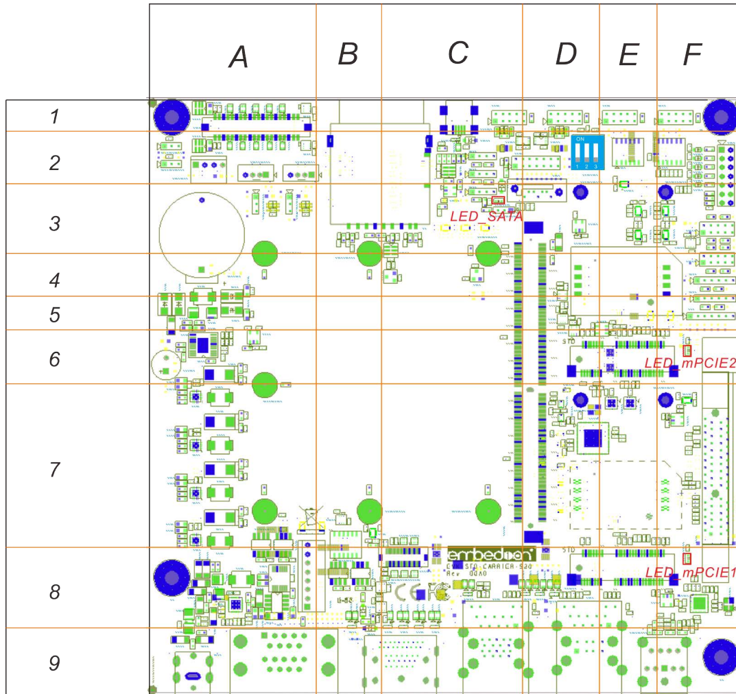
Figure 7: LED Locations
